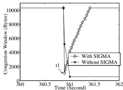
Fig. 9. Congestion window in TGSC.
