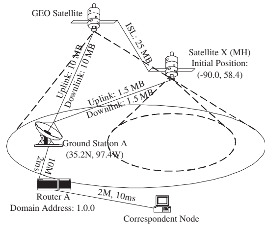
Fig. 4. Mixed LEO-GEO Constellation (MLGC) scenario.
