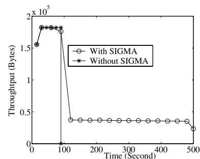
Fig. 8. Throughput in MLGC scenario.
