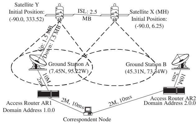
Fig. 2. Two-Ground Station Constellation (TGSC) scenario.
