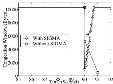
Fig. 10. Congestion window in OGSCI.
