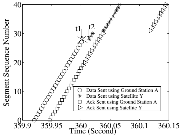
Fig. 5. Packet trace during first Handover in TGSC scenario.
