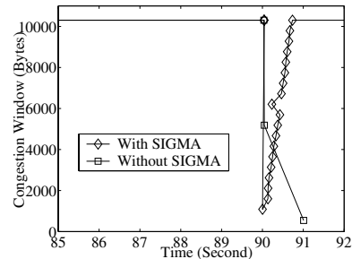
Fig. 11. Congestion Window in MLGC.
