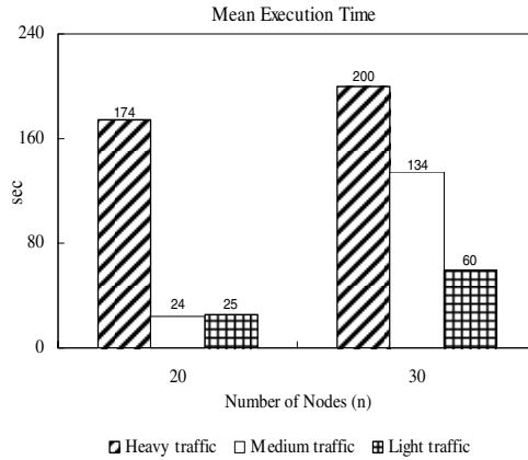
Fig. 2. Mean execution time
