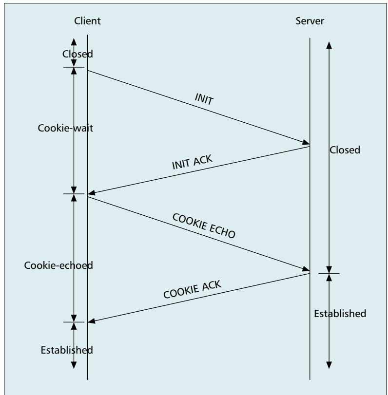
■ Figure 6. SCTP association setup message sequence.
