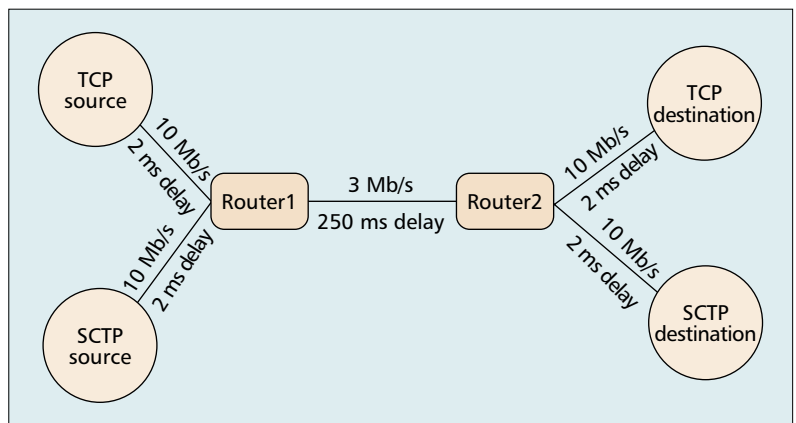
Figure 9. TCP and SCTP sharing a common satellite link.
