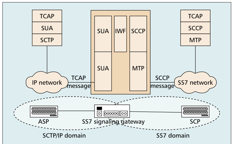
Figure 14. Transport of TCAP messages using SCTP.
