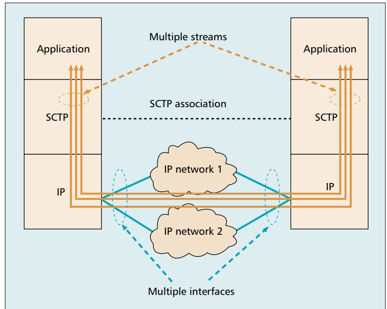
■ Figure 1. A schematic view of an SCTP association.
