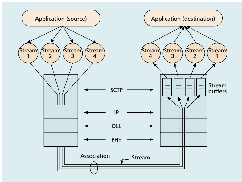
■ Figure 3. An SCTP association consisting of four streams carrying data from one upper layer application.
