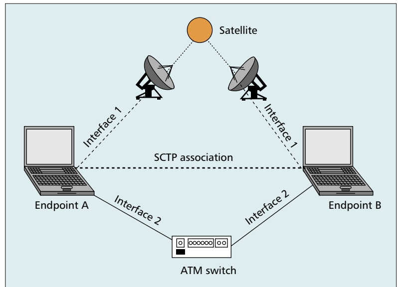
■ Figure 2. An SCTP association with multihomed endpoints.
