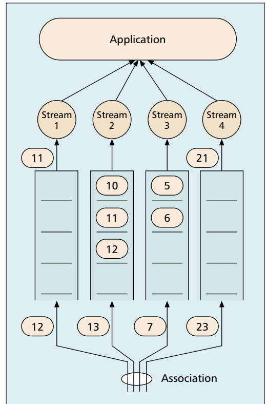
■ Figure 4. An illustration showing HOL blocking of individual streams at the receiver.
