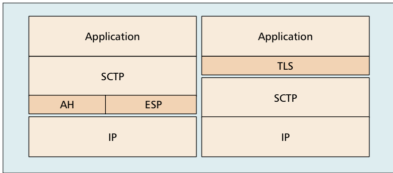
■ Figure 7. Usage of IPSec and TLS with SCTP.
