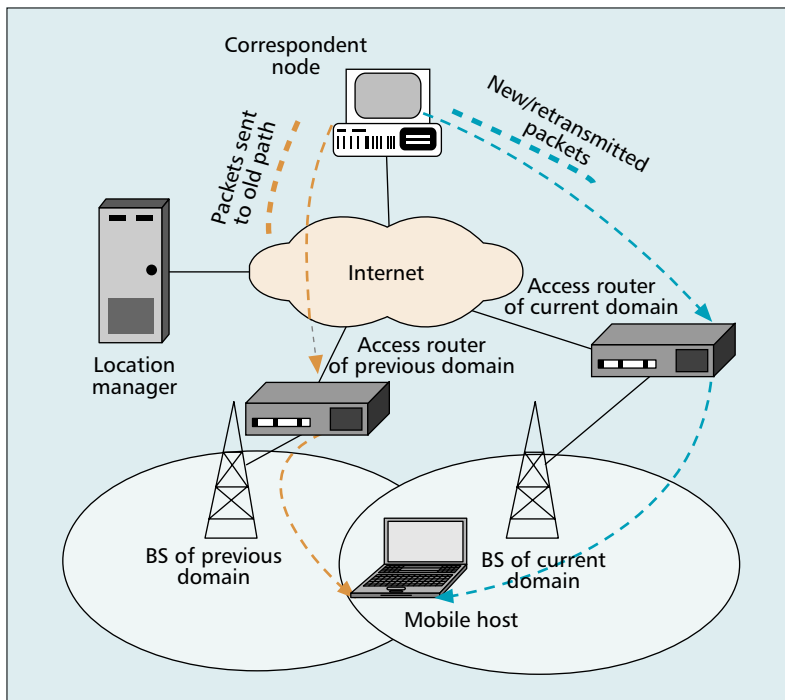
■ Figure 12. Handover in TraSH [14] using SCTP's multihoming.
