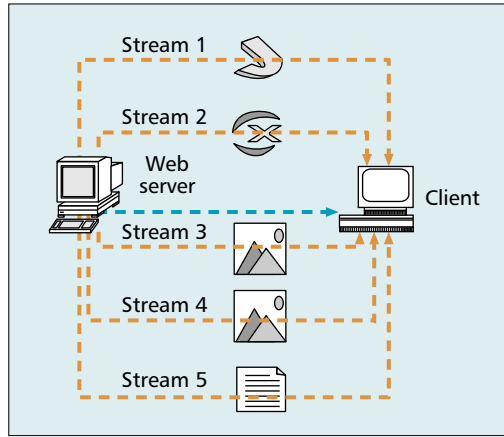
■ Figure 5. Multistreaming in Web browsing.
