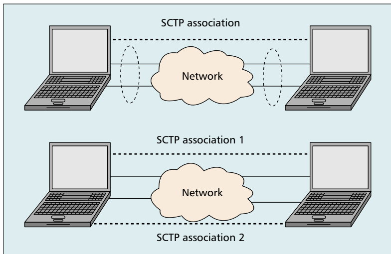
■ Figure 10. Two approaches to link failover protection.
