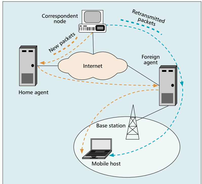
■ Figure 11. Reducing Mobile IP home agent load using SCTP multihoming.
