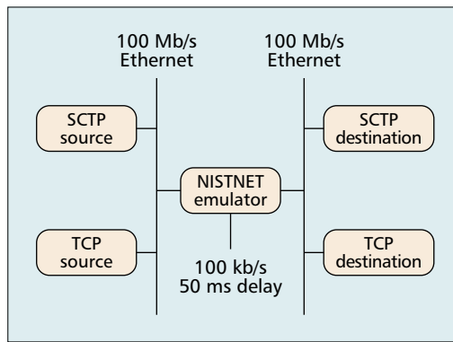
Figure 8. TCP and SCTP sharing a common WAN link.
